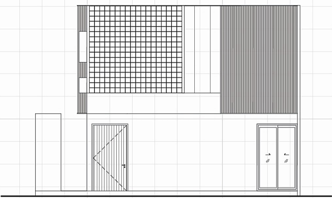
BACK ELEVATION
